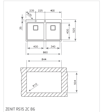
ZENIT RS15 2C 86
