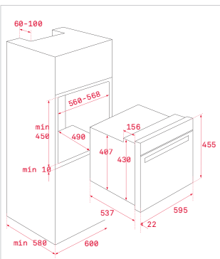
HLC 847 SC - HLC 8400 - HLC 840 HSC 635 - HBC 535
