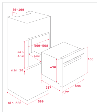
MLC 844 - HLC 844 C - MLC 8440 HSC 644 C
